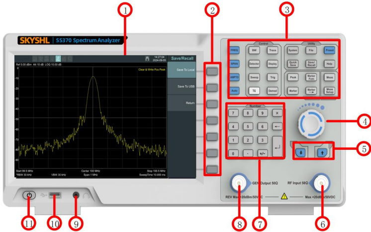
Figure 4- 1 Front panel
