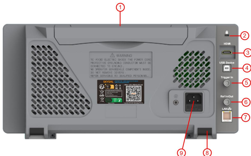
Figure 4- 6 Rear Panel
